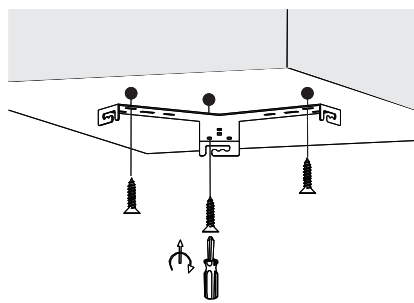
5. Apply screws
